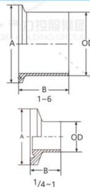
端头 tri-clamp Ferrule
