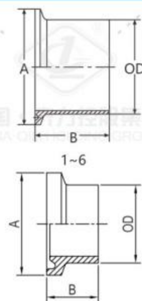
端头 (加长型) Weld Ferrule
