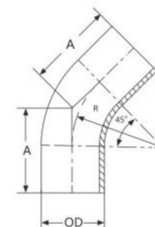
45°长弯头 Weld 45-deg Elbow
