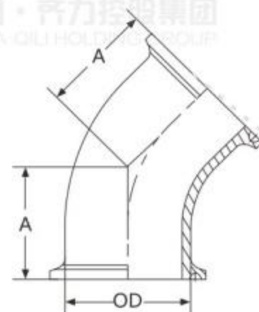
45°卡式弯头 Clamp 45-deg Elbow
