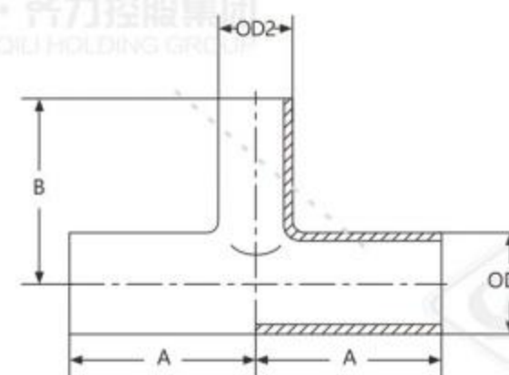
变径长三通 Weld long reducing Tee
