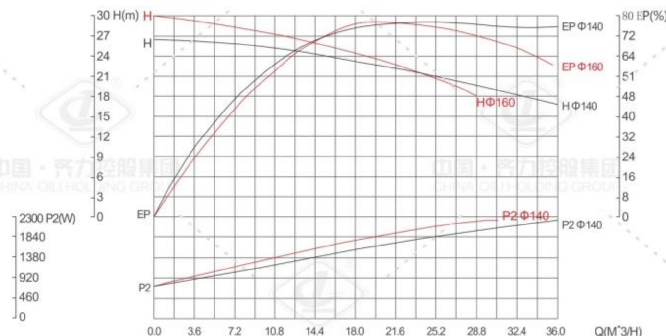
性能曲线 Performance curve
