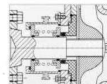
A: 水冷双端面机械密封 Water-cooled double end face mechanical seal
