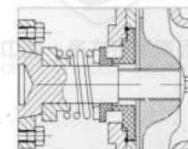
单端面机械密封 Single mechanical seal
