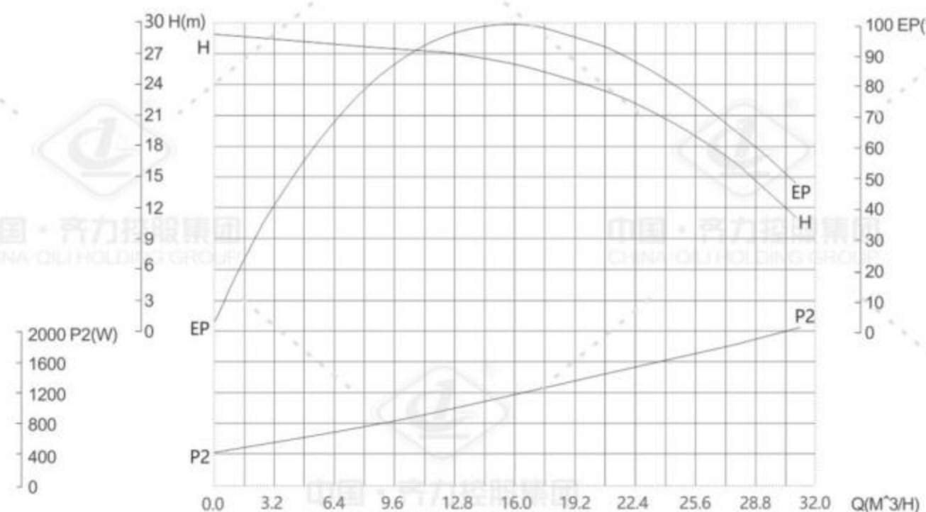
性能曲线 Performance curve
