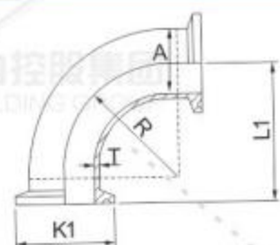
卡箍式弯头90° Clamped Elbow 90°
