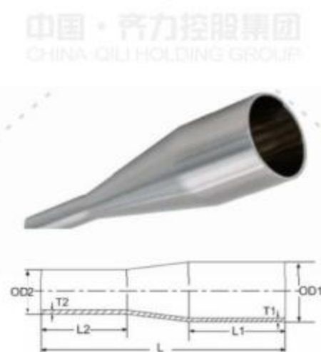
加长同心变径 Concentric Reducer
