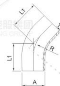
长型焊接式弯头45° Long Welded Elbow 45°
