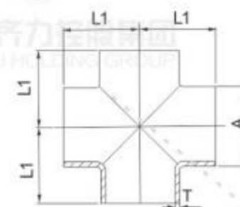
焊接式四通 Welded Cross
