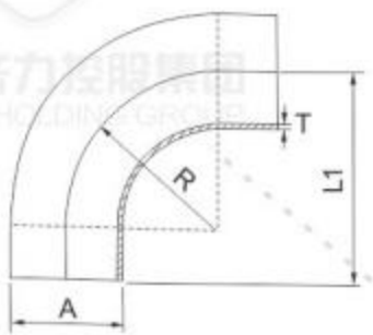
长型焊接式弯头90° Long Welded Elbow 90°
