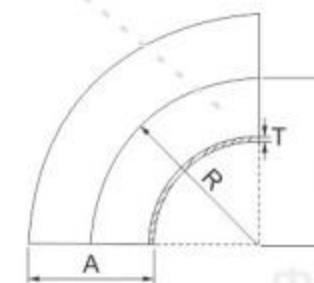
焊接式弯头90° Welded Elbow 90°
