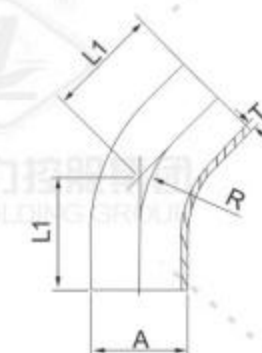
长型焊接弯头45° Long Welded Elbow 45°
