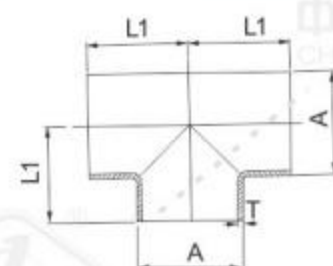
短型焊接式三通 Short Welded Tee
