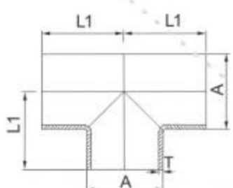
长型焊接式三通 Long Welded Tee
